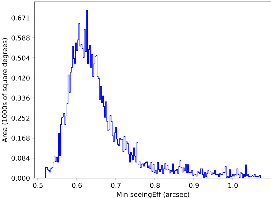
too_elab_r64_d3_ugrizy_v3.4_10yrs Yr 1 all bands: Min seeingEff
