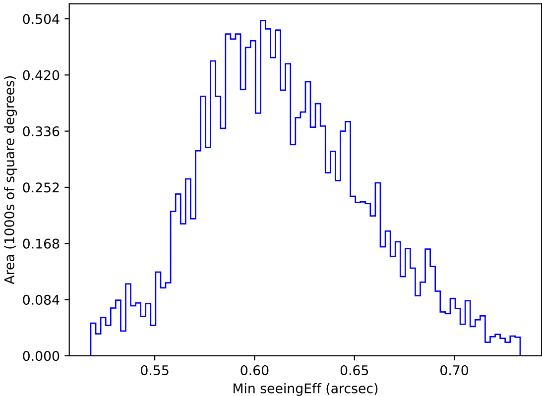
too_elab_r64_d3_ugrizy_v3.4_10yrs WFD z band: Min seeingEff
