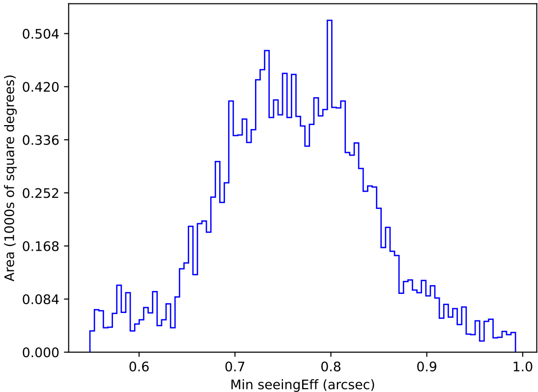
too_elab_r64_d3_ugrizy_v3.4_10yrs WFD u band: Min seeingEff
