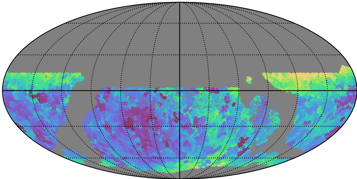
too_elab_r64_d3_ugrizy_v3.4_10yrs WFD r band: Min seeingEff
