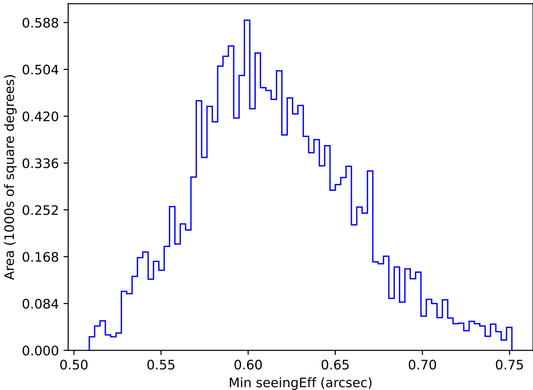
too_elab_r64_d3_ugrizy_v3.4_10yrs WFD r band: Min seeingEff
