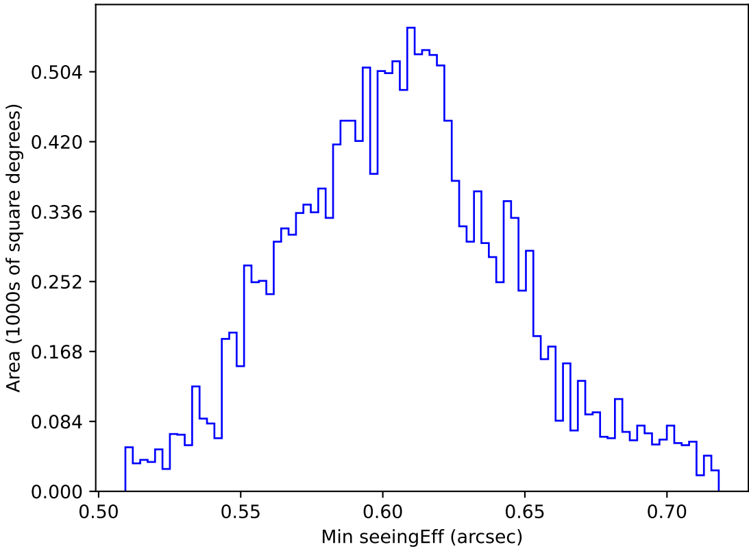
too_elab_r64_d3_ugrizy_v3.4_10yrs WFD i band: Min seeingEff
