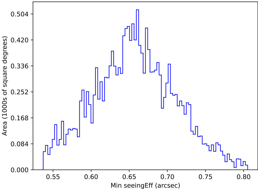
too_elab_r64_d3_ugrizy_v3.4_10yrs WFD g band: Min seeingEff
