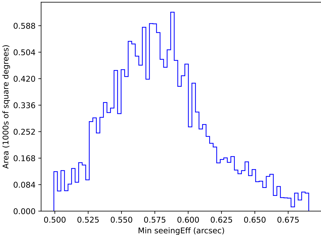
too_elab_r64_d3_ugrizy_v3.4_10yrs WFD all bands: Min seeingEff
