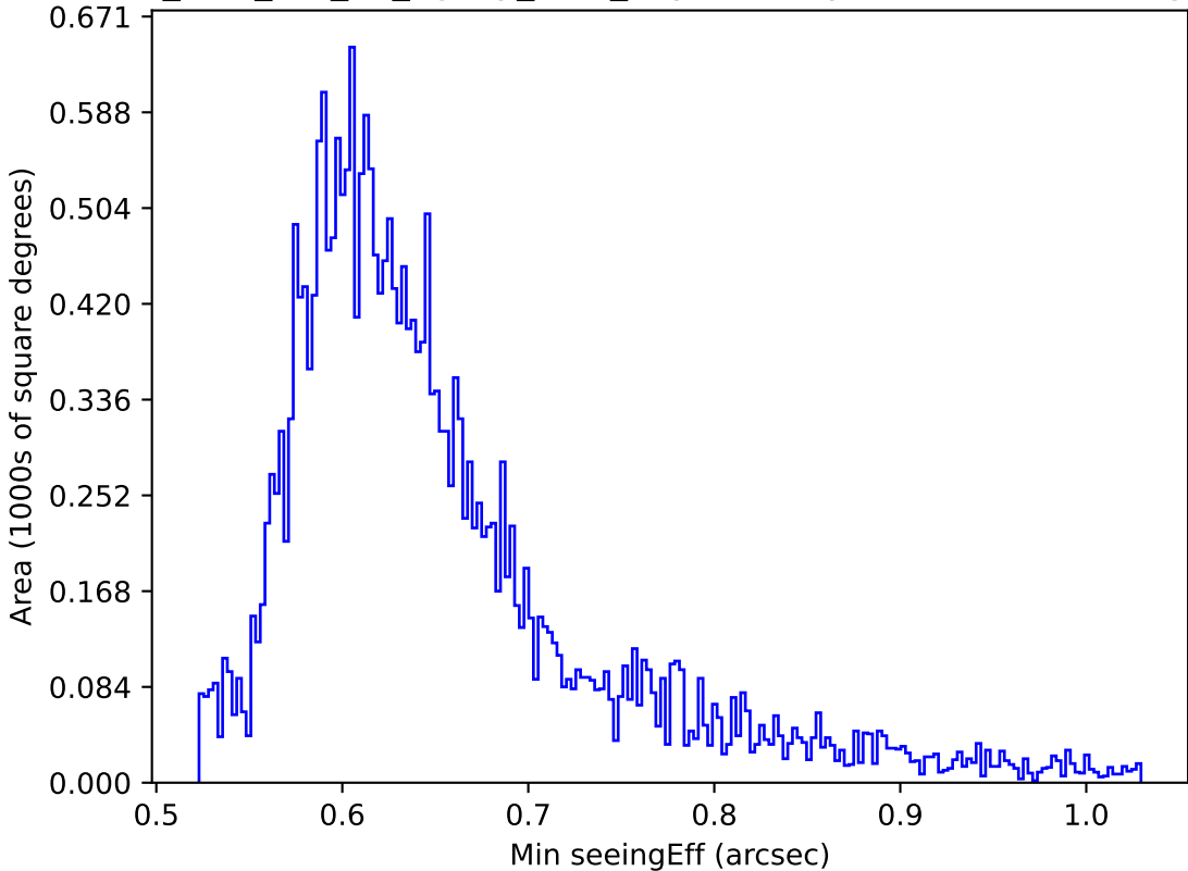
too_elab_r64_d3_ugrizy_v3.4_10yrs All sky z band: Min seeingEff
