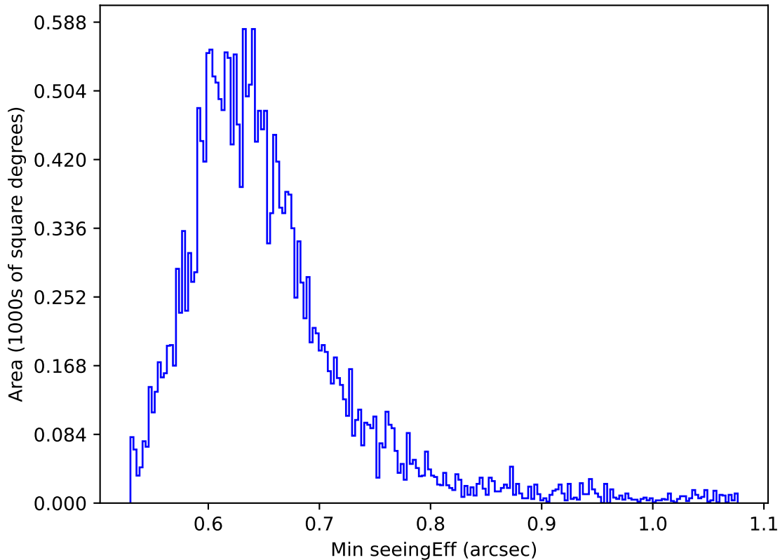
too_elab_r64_d3_ugrizy_v3.4_10yrs All sky y band: Min seeingEff
