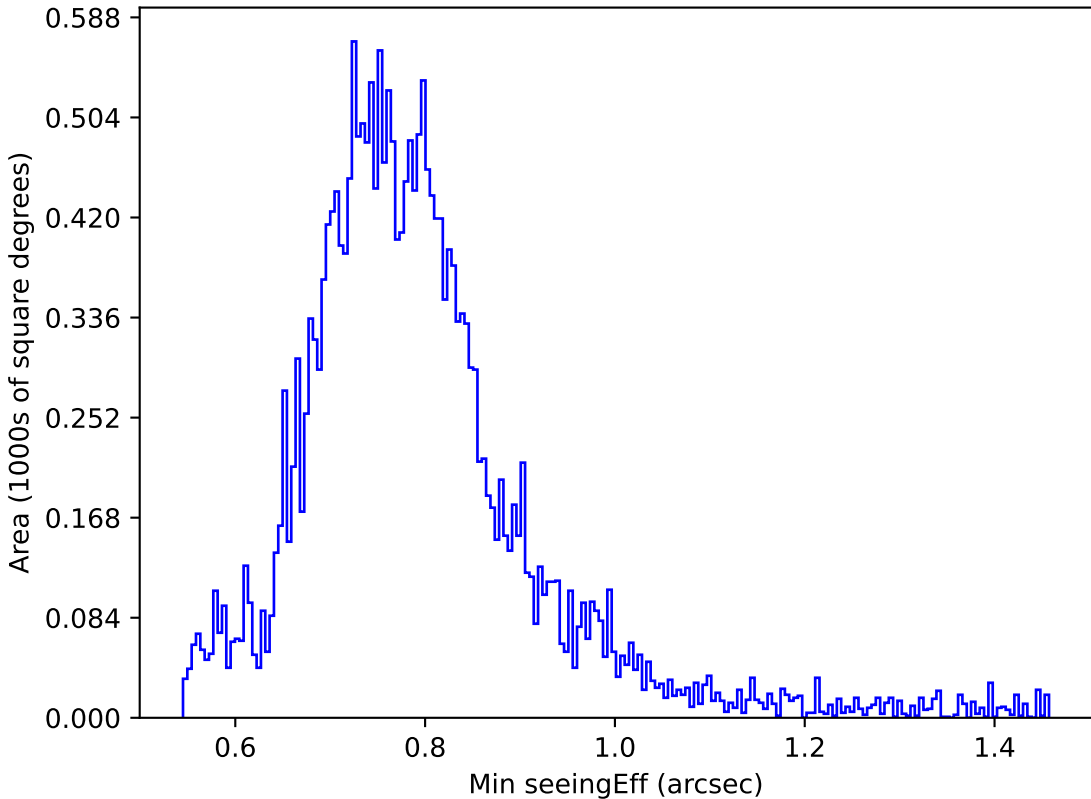
too_elab_r64_d3_ugrizy_v3.4_10yrs All sky u band: Min seeingEff
