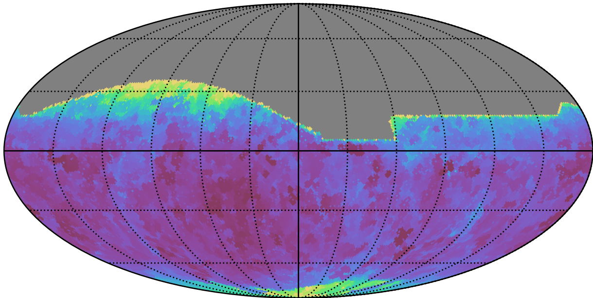
too_elab_r64_d3_ugrizy_v3.4_10yrs All sky r band: Min seeingEff
