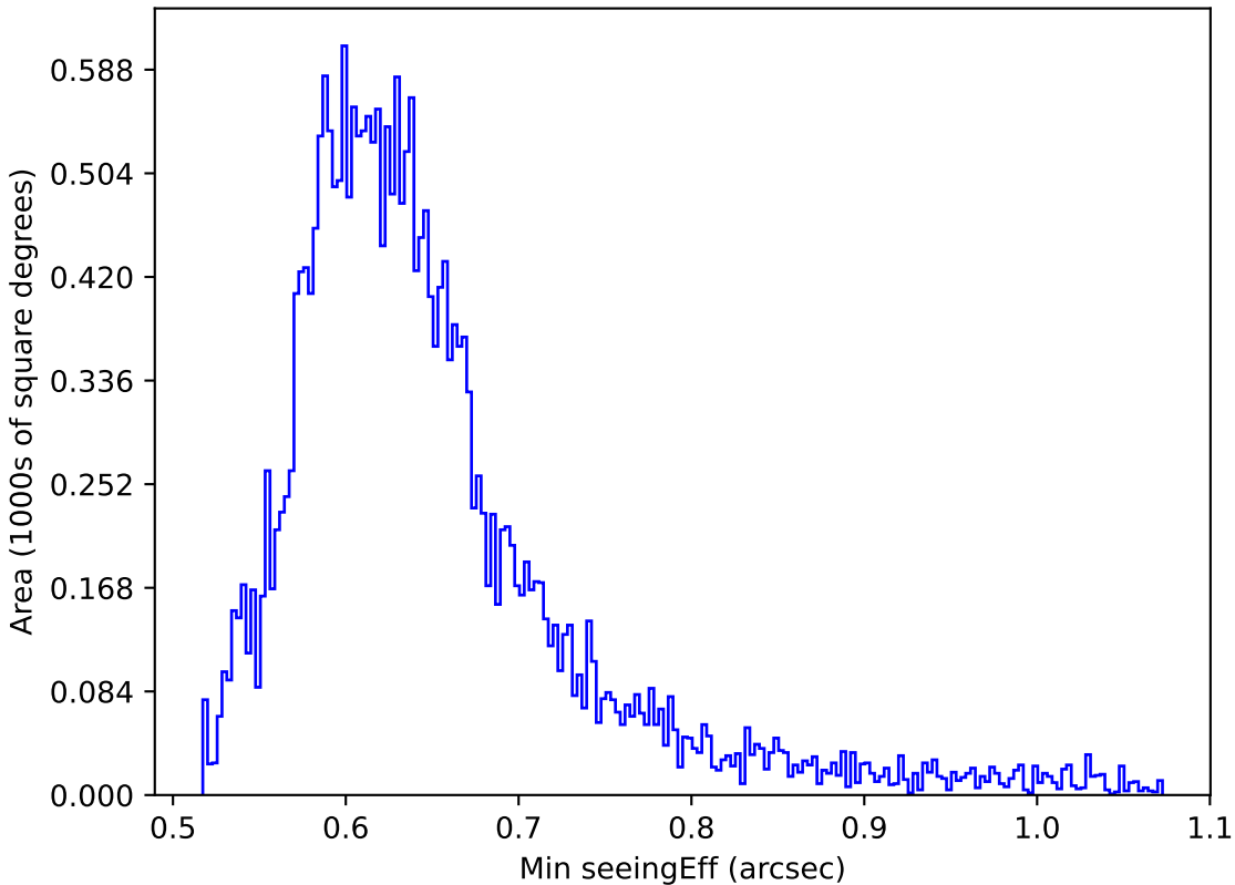
too_elab_r64_d3_ugrizy_v3.4_10yrs All sky r band: Min seeingEff
