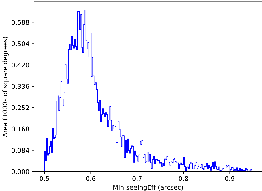
too_elab_r64_d3_ugrizy_v3.4_10yrs All sky all bands: Min seeingEff
