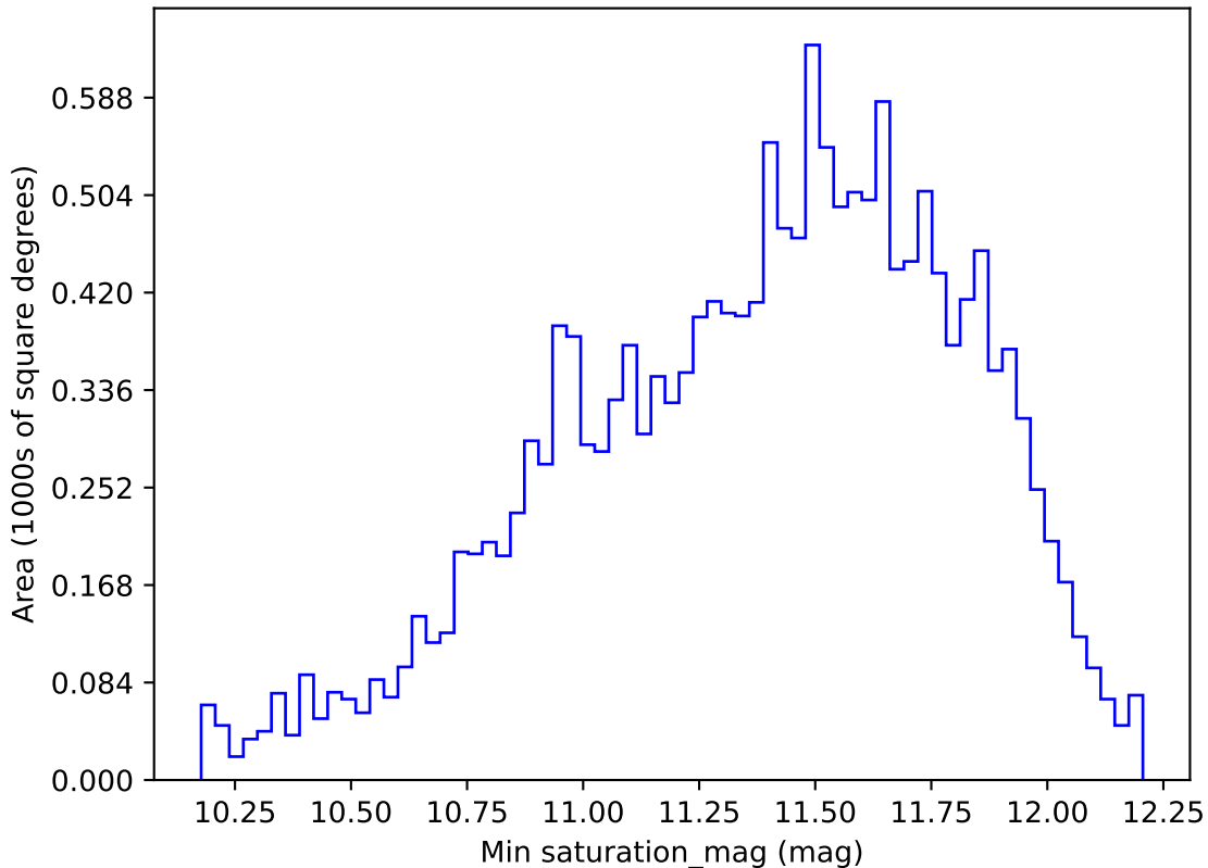
too_elab_r64_d3_ugrizy_v3.4_10yrs WFD u band: Min saturation_mag
