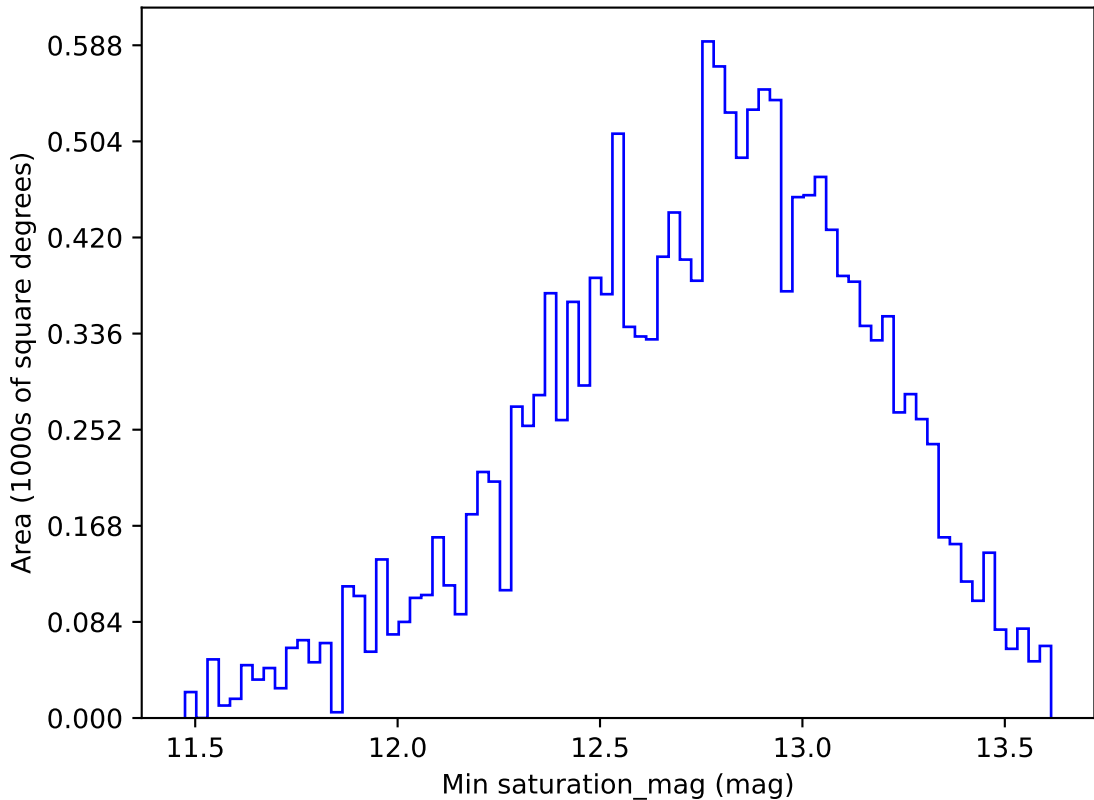
too_elab_r64_d3_ugrizy_v3.4_10yrs WFD g band: Min saturation_mag
