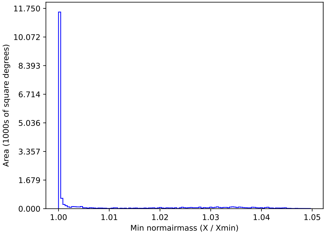
too_elab_r64_d3_ugrizy_v3.4_10yrs WFD g band: Min normairmass
