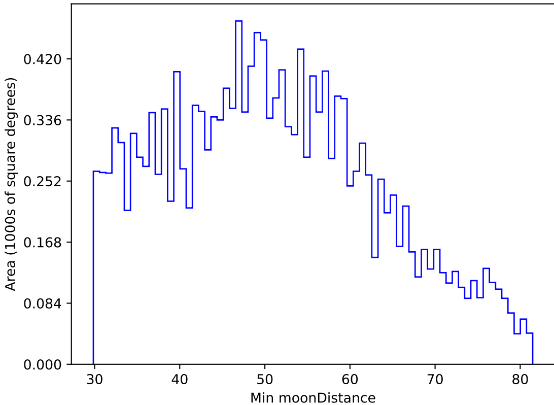
too_elab_r64_d3_ugrizy_v3.4_10yrs WFD u band: Min moonDistance
