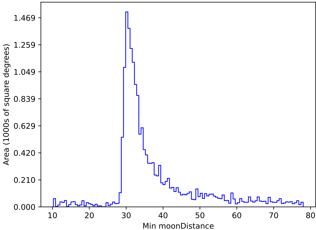
too_elab_r64_d3_ugrizy_v3.4_10yrs WFD r band: Min moonDistance
