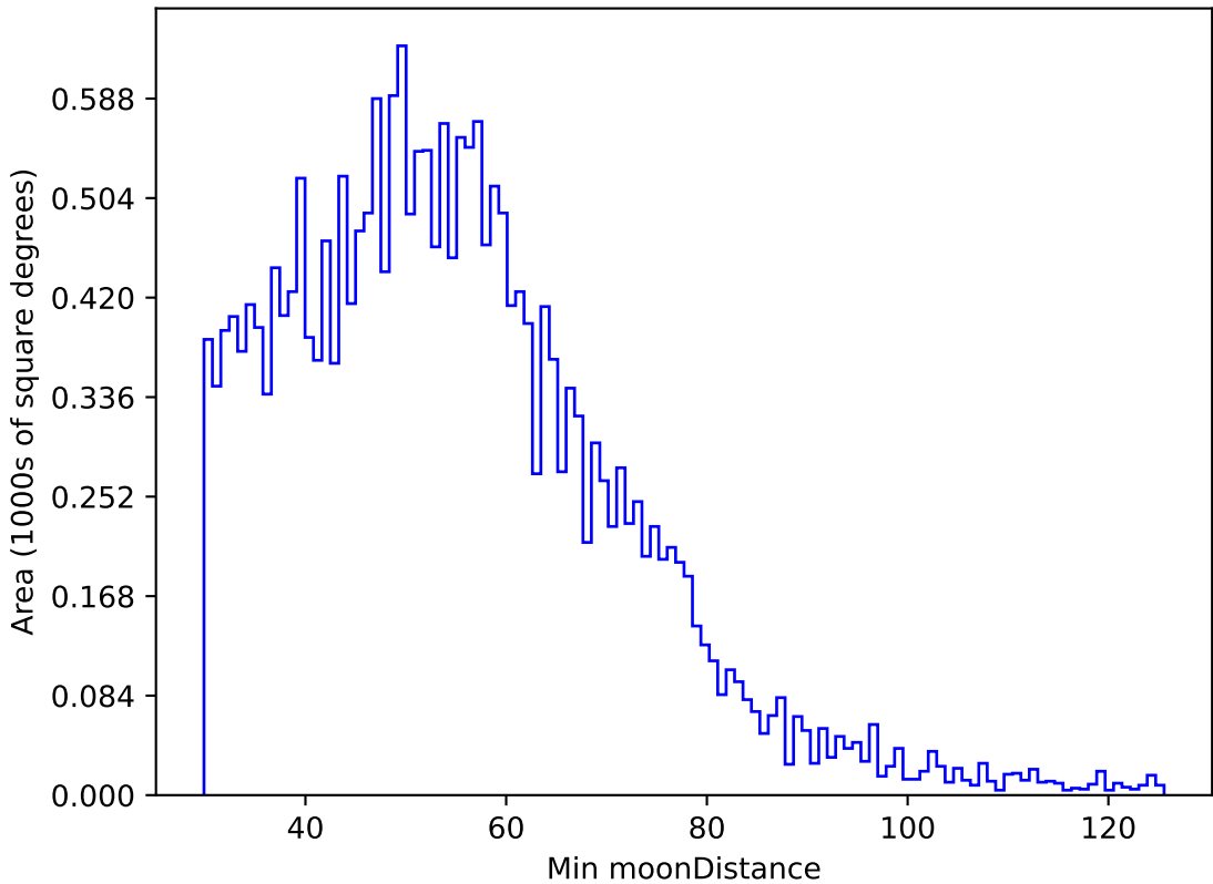
too_elab_r64_d3_ugrizy_v3.4_10yrs All sky u band: Min moonDistance
