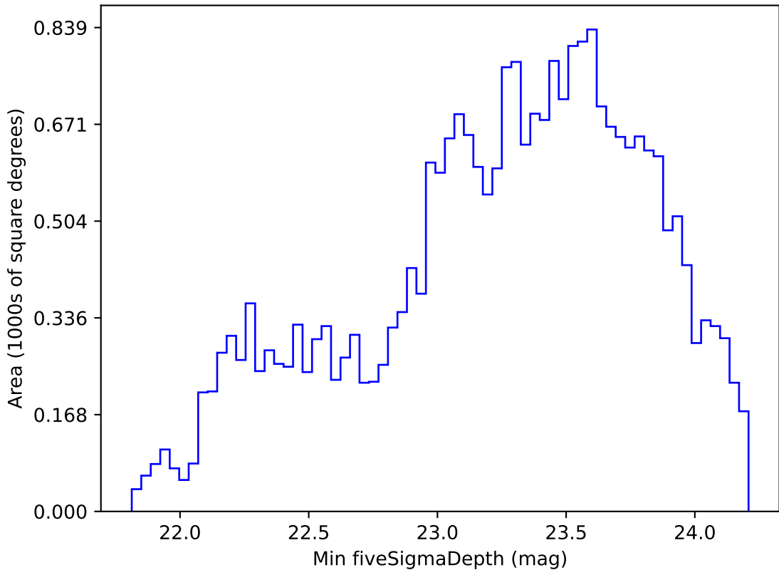
too_elab_r64_d3_ugrizy_v3.4_10yrs Yr 1 r band: Min fiveSigmaDepth
