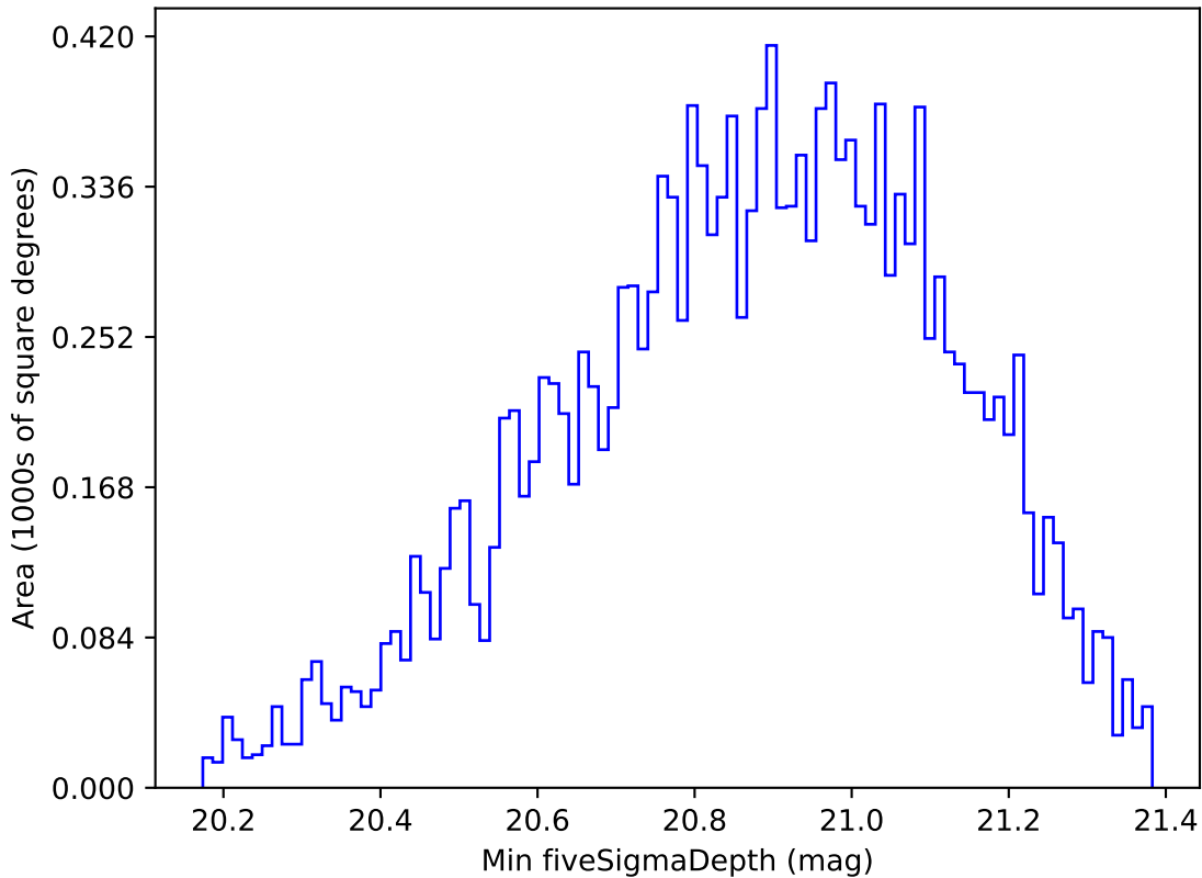
too_elab_r64_d3_ugrizy_v3.4_10yrs WFD y band: Min fiveSigmaDepth
