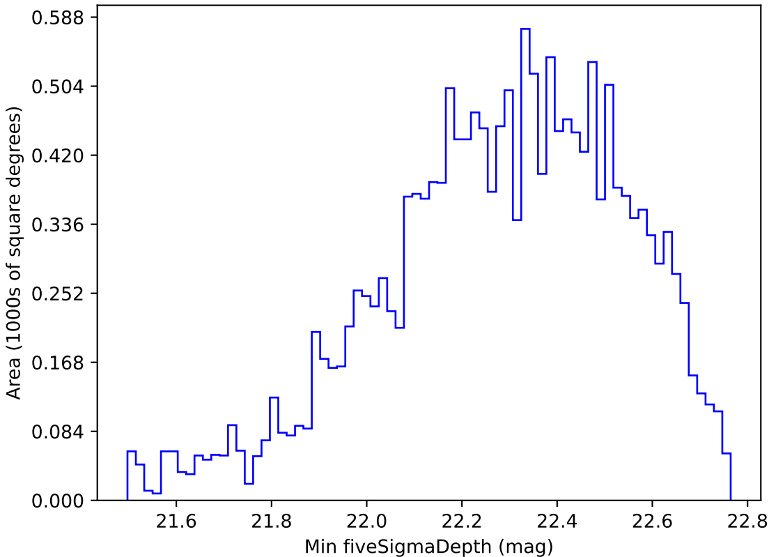
too_elab_r64_d3_ugrizy_v3.4_10yrs WFD u band: Min fiveSigmaDepth
