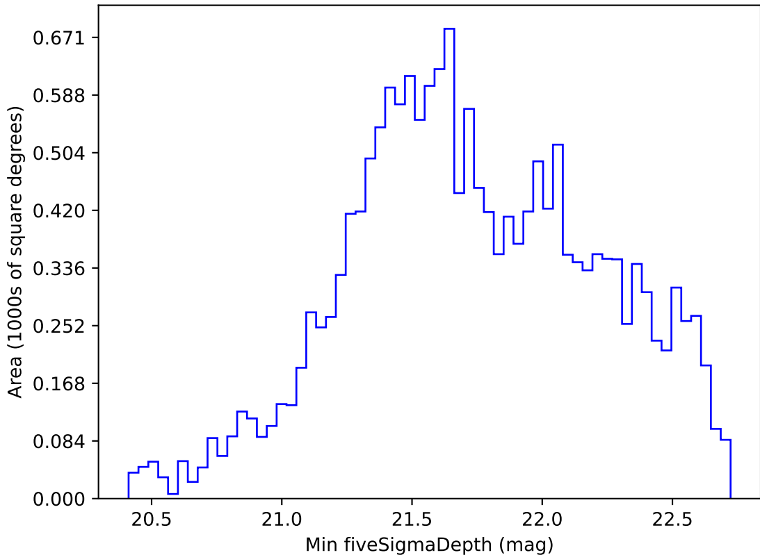
too_elab_r64_d3_ugrizy_v3.4_10yrs WFD i band: Min fiveSigmaDepth
