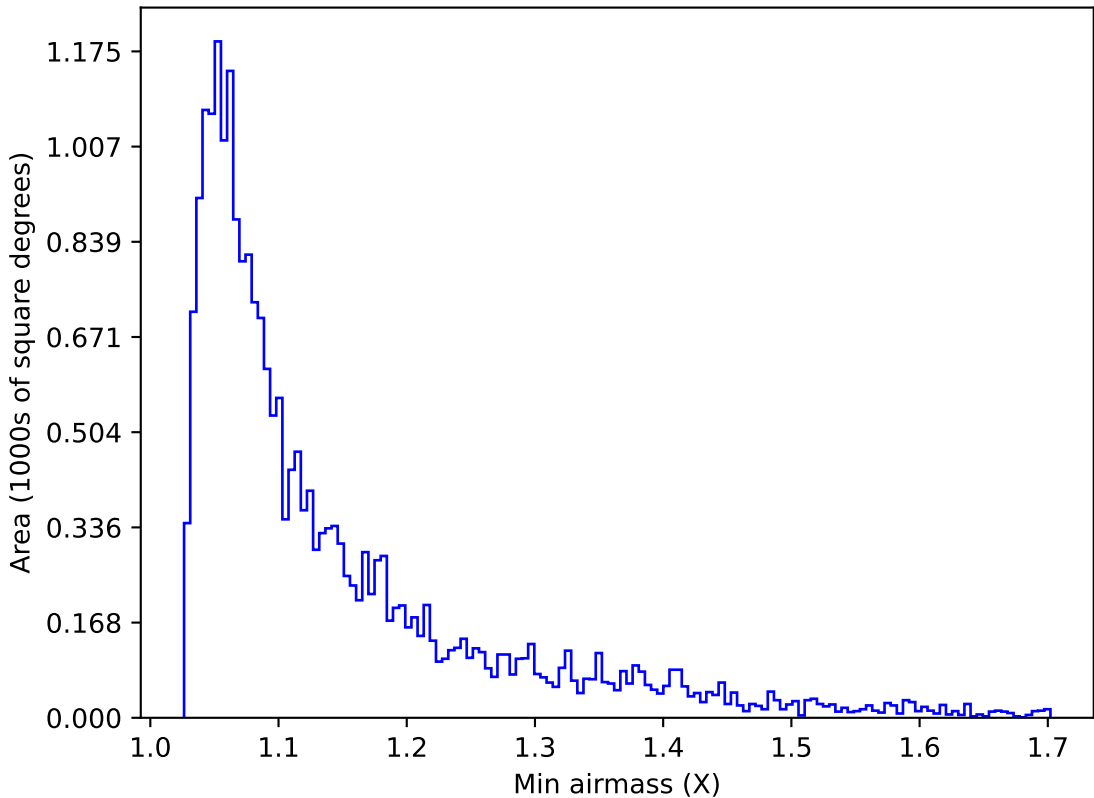
too_elab_r64_d3_ugrizy_v3.4_10yrs Yr 1 u band: Min airmass
