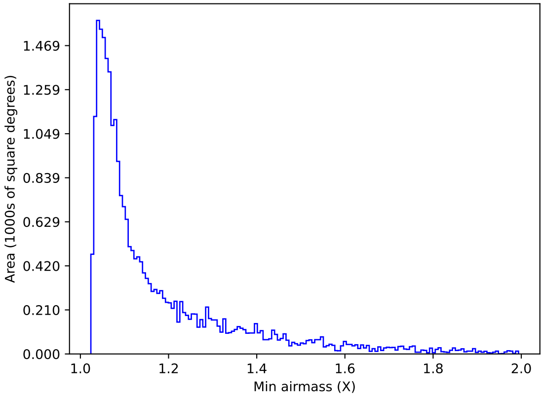
too_elab_r64_d3_ugrizy_v3.4_10yrs Yr 1 g band: Min airmass
