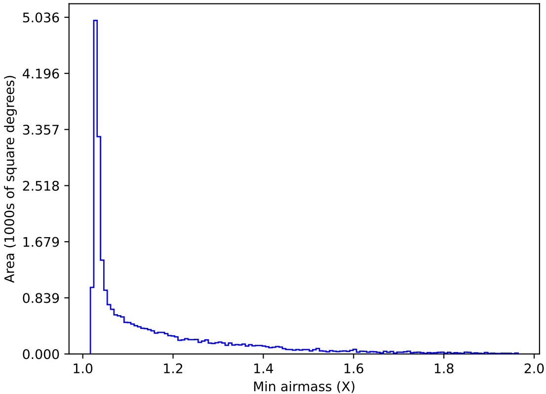
too_elab_r64_d3_ugrizy_v3.4_10yrs Yr 1 all bands: Min airmass
