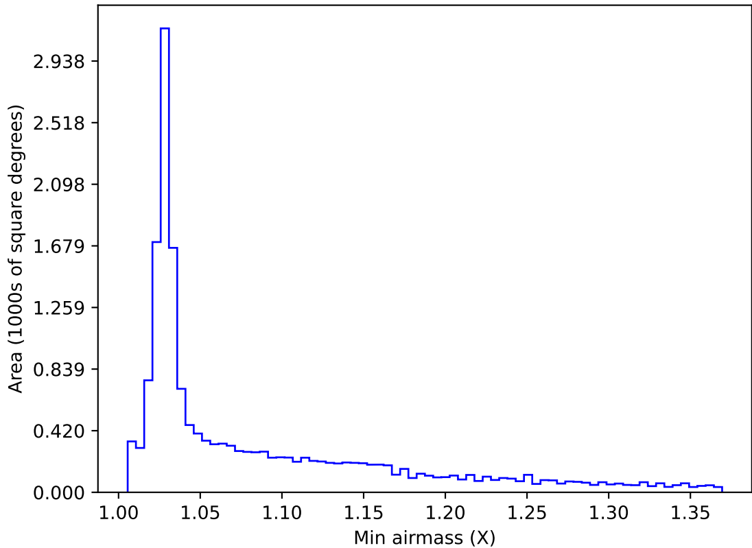
too_elab_r64_d3_ugrizy_v3.4_10yrs WFD z band: Min airmass
