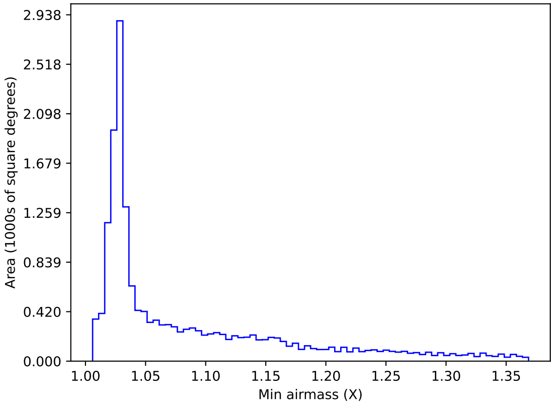
too_elab_r64_d3_ugrizy_v3.4_10yrs WFD r band: Min airmass
