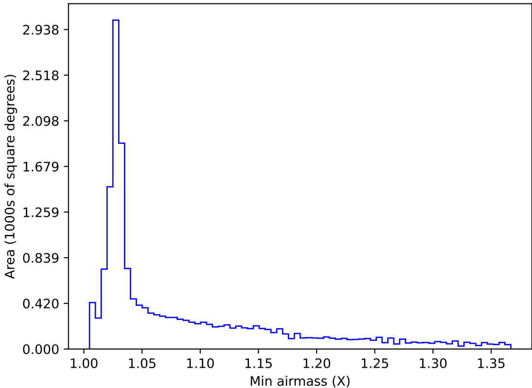
too_elab_r64_d3_ugrizy_v3.4_10yrs WFD i band: Min airmass
