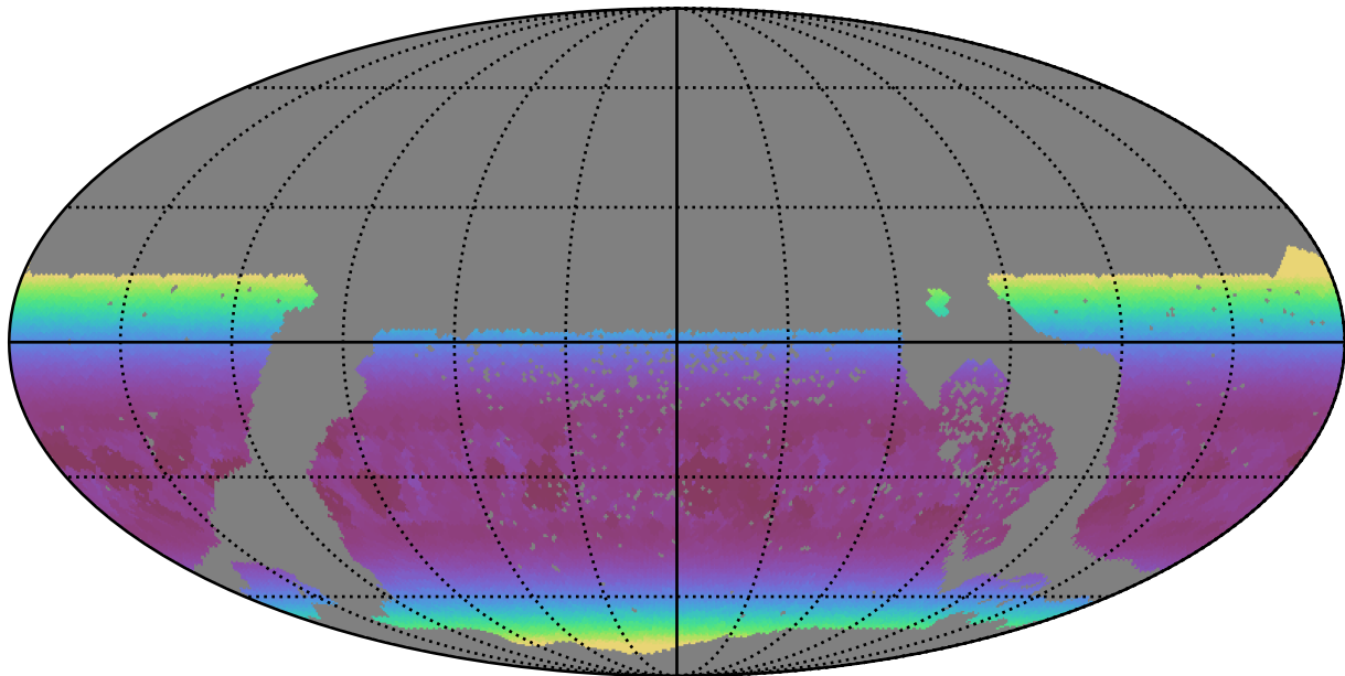
too_elab_r64_d3_ugrizy_v3.4_10yrs WFD g band: Min airmass
