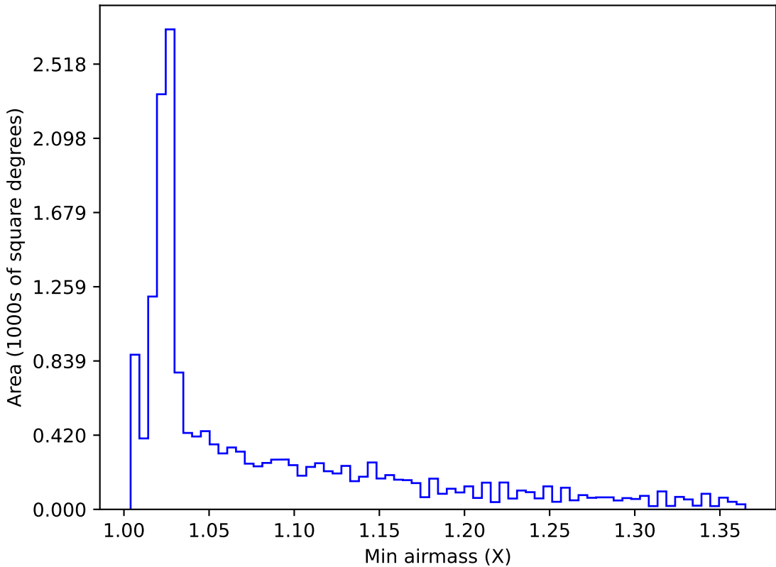
too_elab_r64_d3_ugrizy_v3.4_10yrs WFD all bands: Min airmass
