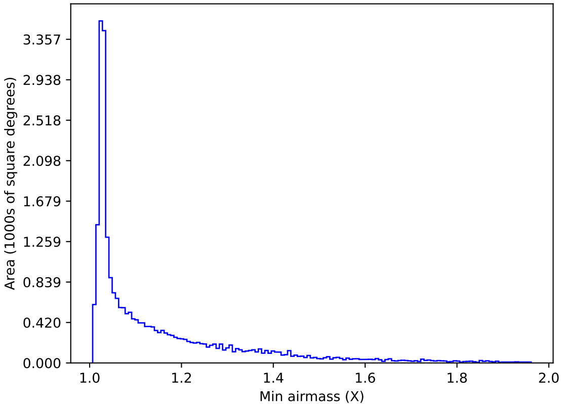
too_elab_r64_d3_ugrizy_v3.4_10yrs All sky r band: Min airmass
