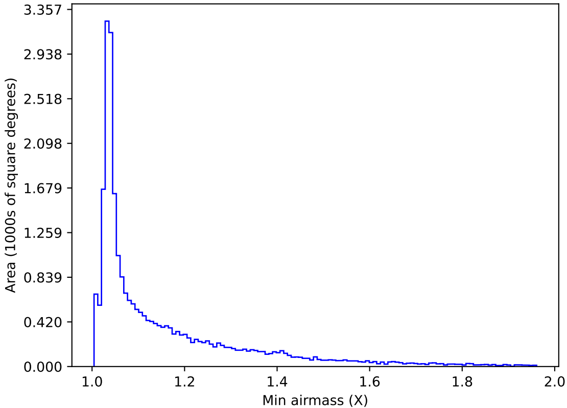
too_elab_r64_d3_ugrizy_v3.4_10yrs All sky g band: Min airmass
