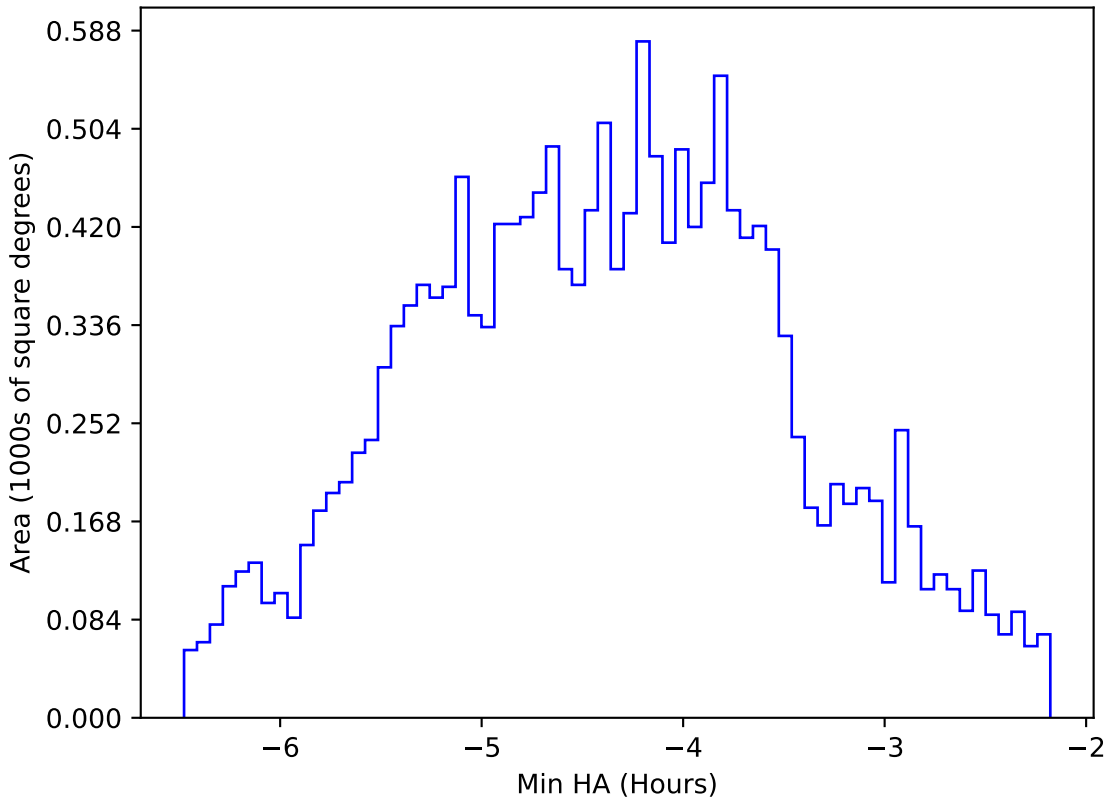
too_elab_r64_d3_ugrizy_v3.4_10yrs WFD z band: Min HA
