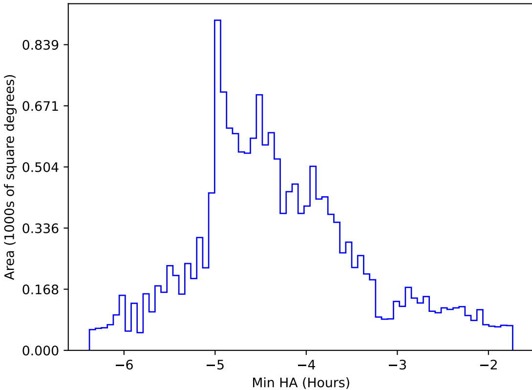
too_elab_r64_d3_ugrizy_v3.4_10yrs WFD g band: Min HA
