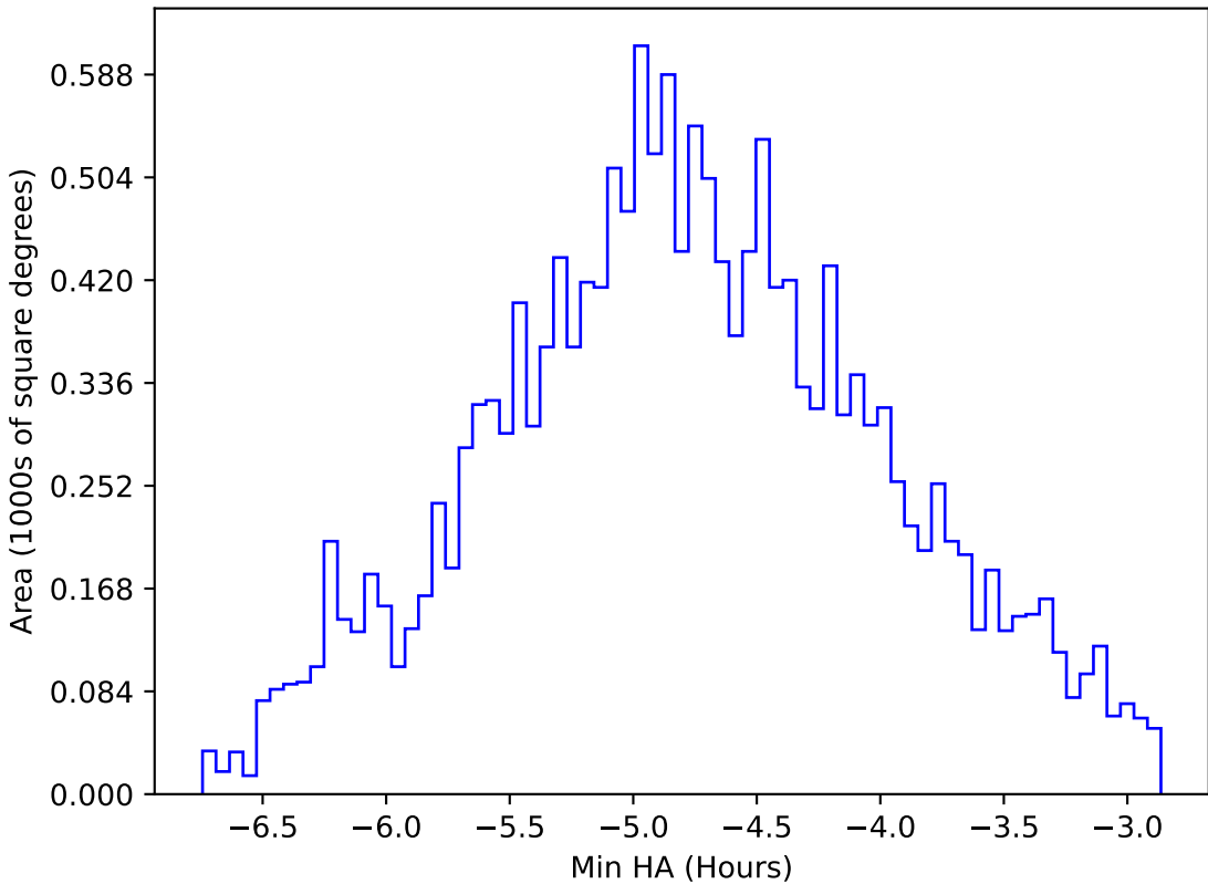
too_elab_r64_d3_ugrizy_v3.4_10yrs WFD all bands: Min HA
