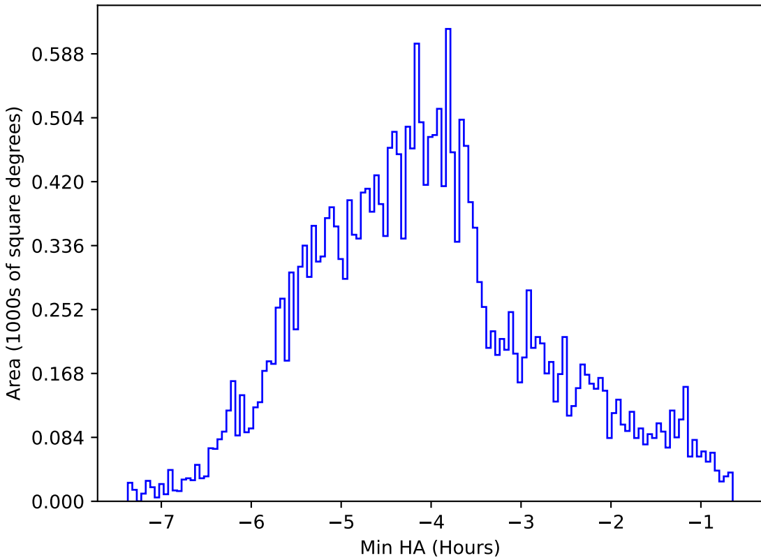
too_elab_r64_d3_ugrizy_v3.4_10yrs All sky z band: Min HA
