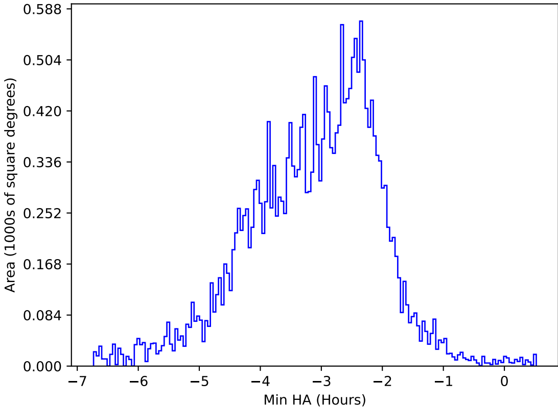
too_elab_r64_d3_ugrizy_v3.4_10yrs All sky u band: Min HA
