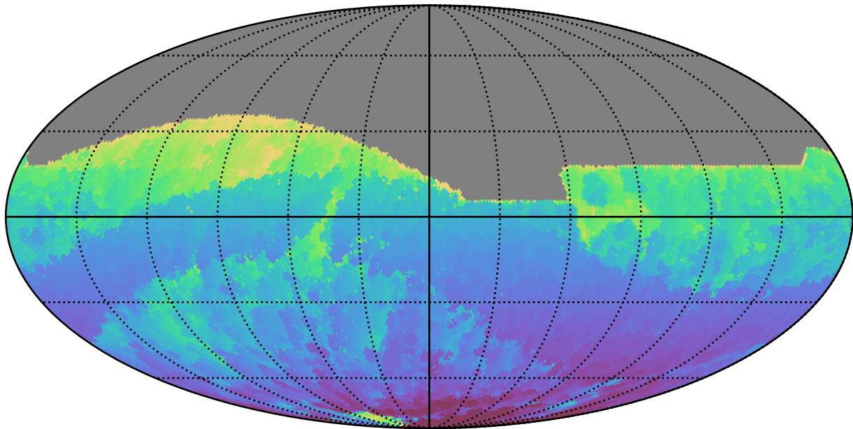
too_elab_r64_d3_ugrizy_v3.4_10yrs All sky r band: Min HA
