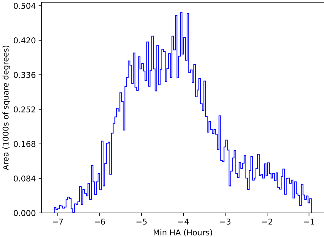
too_elab_r64_d3_ugrizy_v3.4_10yrs All sky r band: Min HA
