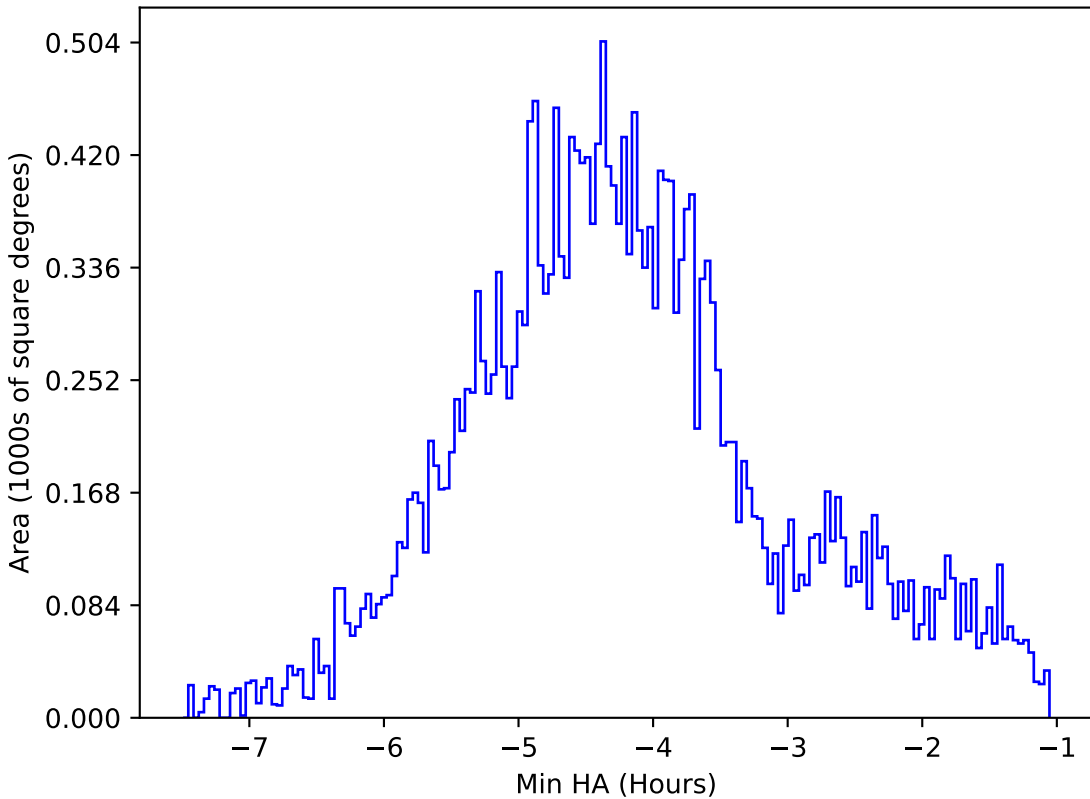
too_elab_r64_d3_ugrizy_v3.4_10yrs All sky i band: Min HA
