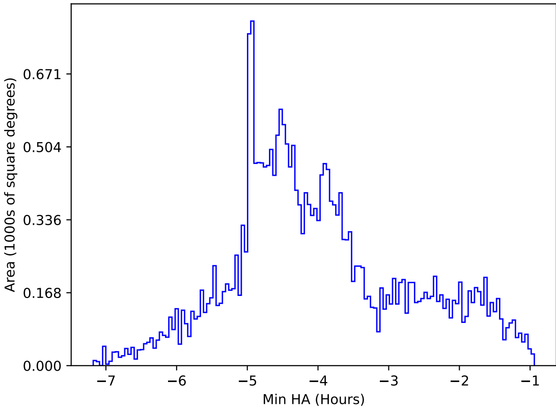
too_elab_r64_d3_ugrizy_v3.4_10yrs All sky g band: Min HA
