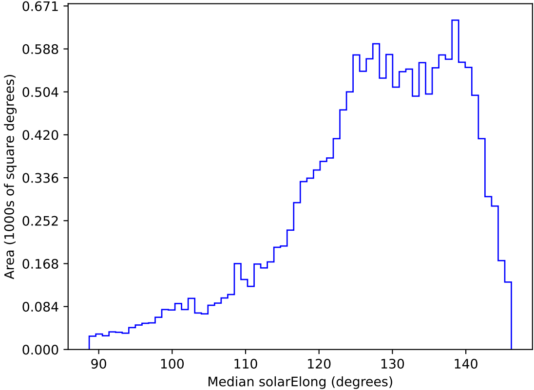
too_elab_r64_d3_ugrizy_v3.4_10yrs WFD z band: Median solarElong
