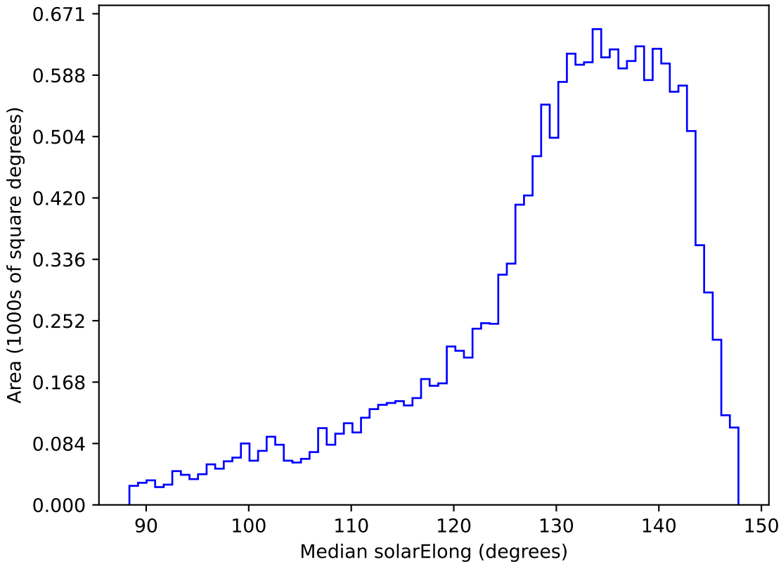
too_elab_r64_d3_ugrizy_v3.4_10yrs WFD y band: Median solarElong
