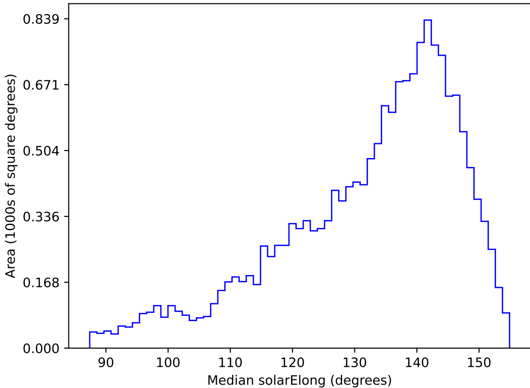
too_elab_r64_d3_ugrizy_v3.4_10yrs WFD u band: Median solarElong
