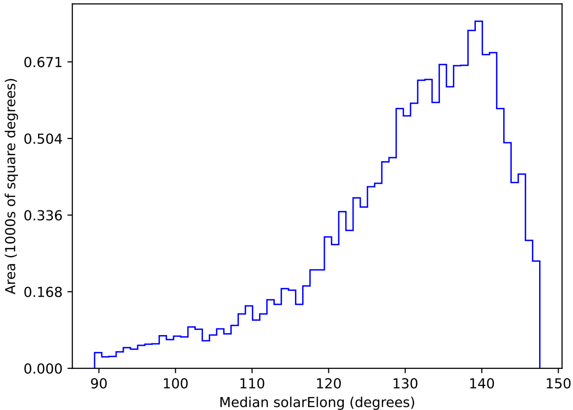
too_elab_r64_d3_ugrizy_v3.4_10yrs WFD r band: Median solarElong
