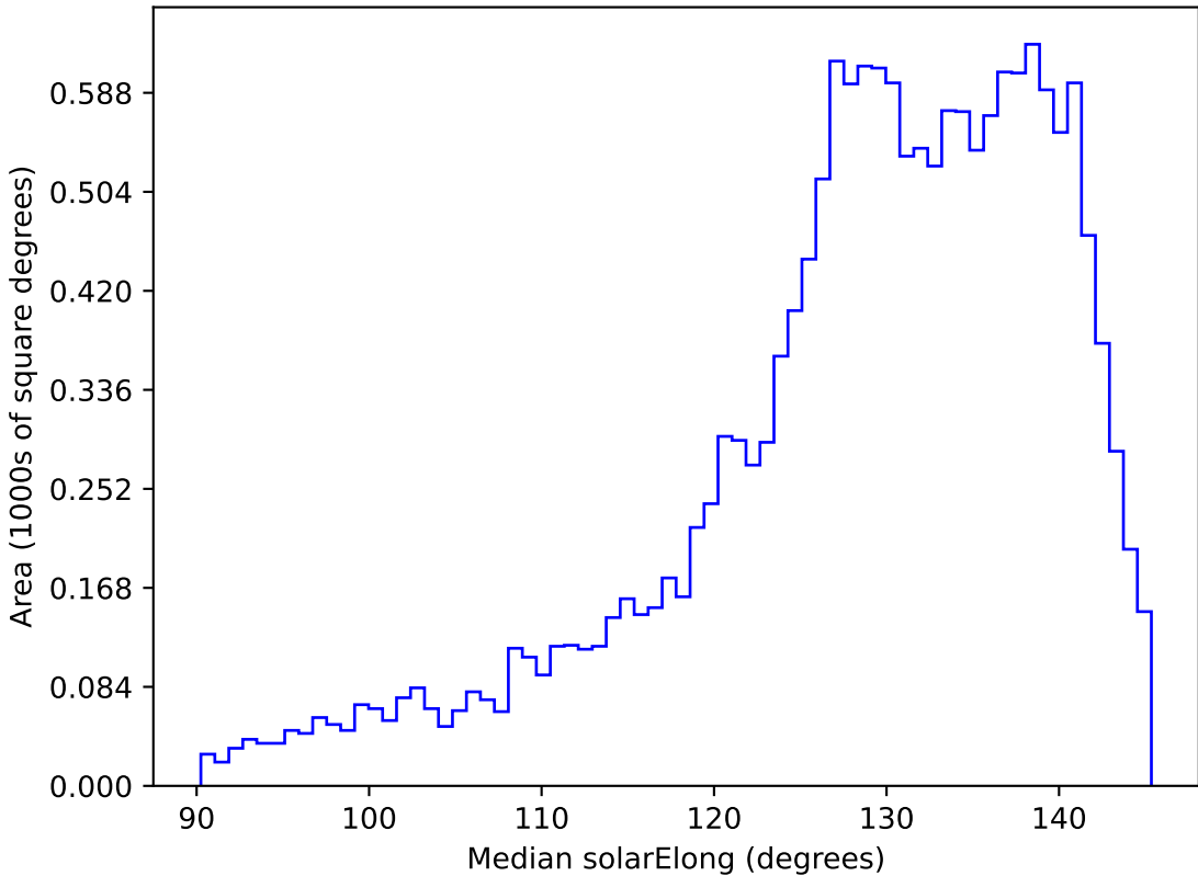
too_elab_r64_d3_ugrizy_v3.4_10yrs WFD i band: Median solarElong
