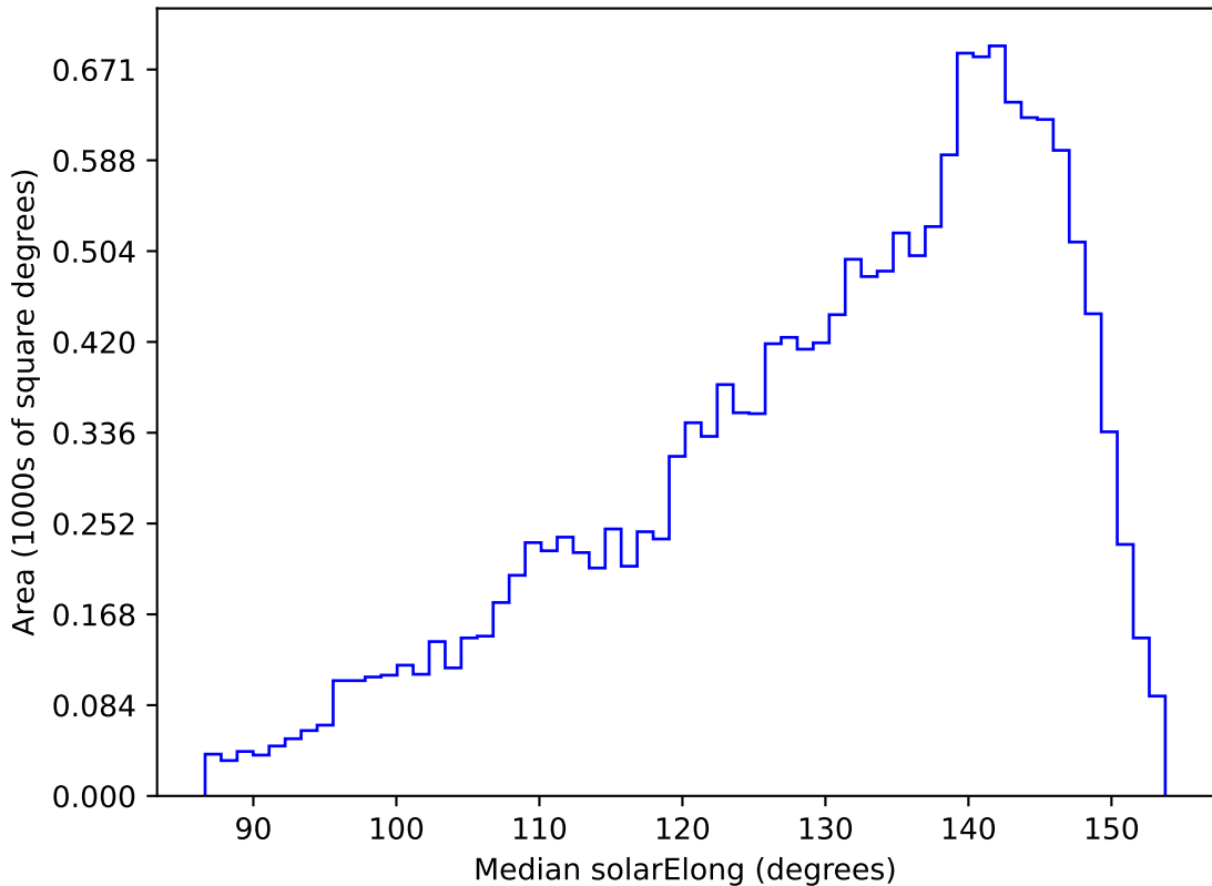
too_elab_r64_d3_ugrizy_v3.4_10yrs WFD g band: Median solarElong
