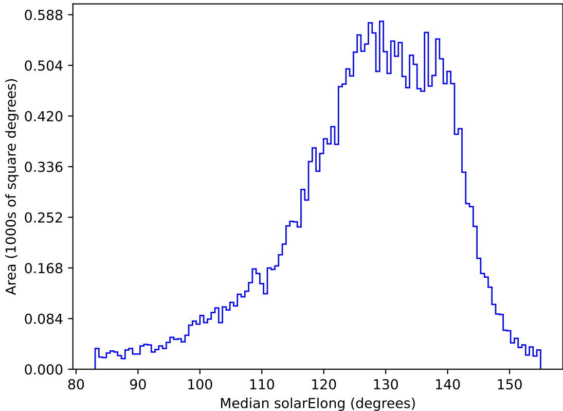
too_elab_r64_d3_ugrizy_v3.4_10yrs All sky z band: Median solarElong
